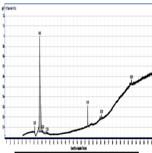
Fig.7. GC-MS Chromatogram of sub-fraction C 3
