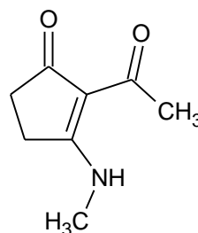
(VI) 2-Acetyl-3-methylaminocyclopentenone
