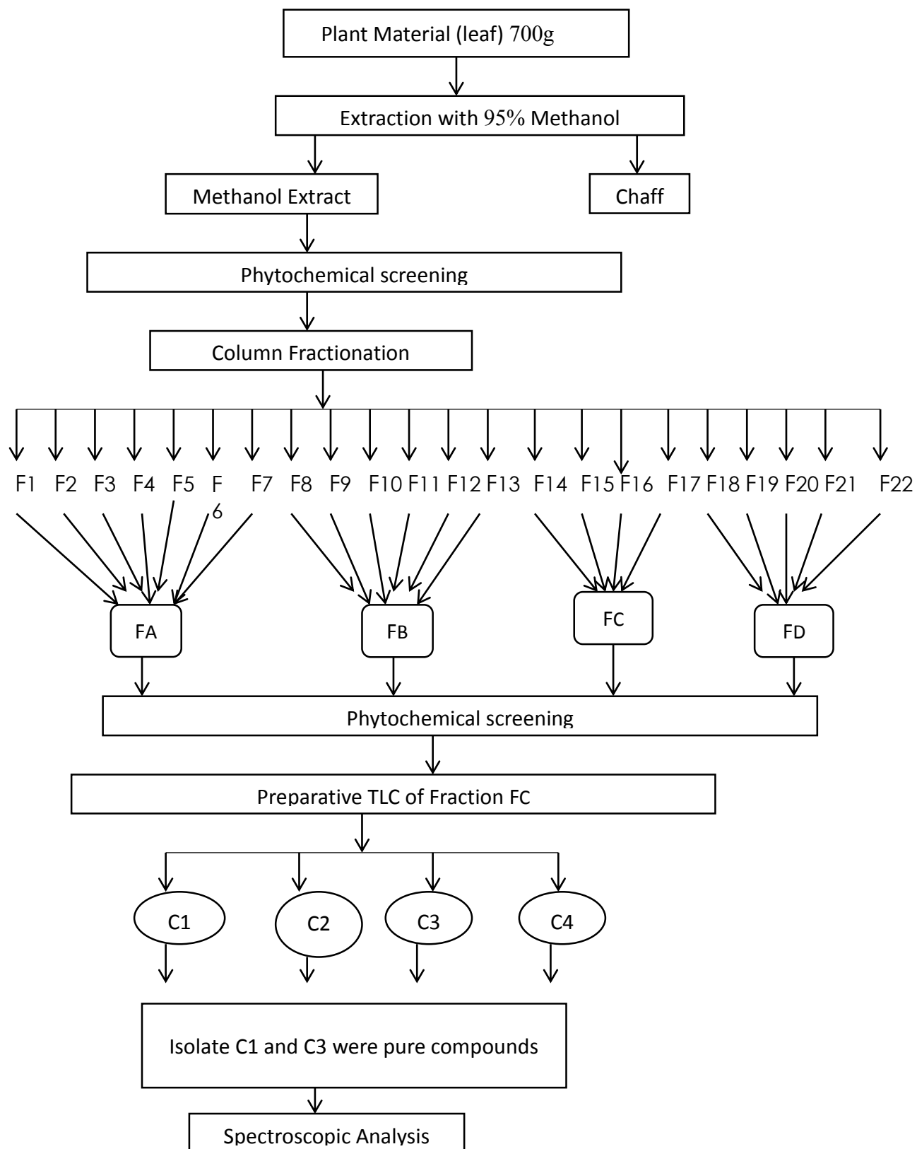
Figure 1. Extraction , Purification scheme of the leaf extract of Ficus sycomorus
