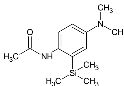
(V) 4'-dimethylamino-2'-(trimethylsilyl)acetanilide
