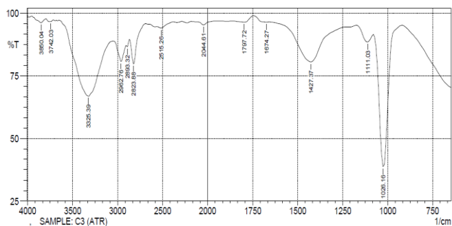
Fig 4. IR Spectra Analysis of Sub-fraction C 3
