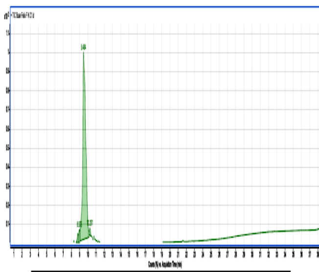
Fig.6. GC-MS Chromatogram of sub-fraction C 1 obtained from F c
