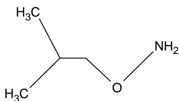
(I) O-(2-methylpropyl)-Hydroxylamine
