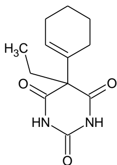
(II) Cyclobarbital
