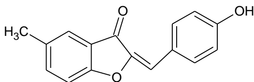
(IX) 5-methyl-4-hydroxyl-2-benzylidene-coumaran-3-one
