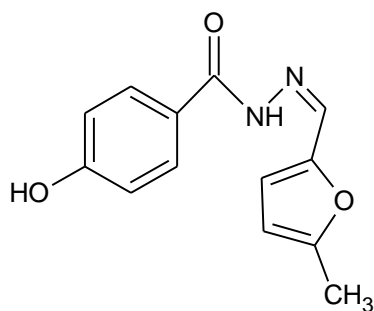
(VII) 5-Methyl-4-hydroxybenzoylhydrazonefurfurol
