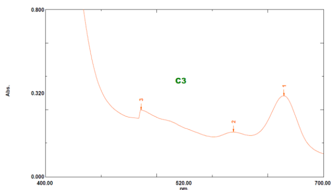
Fig 5. UV Spectra Analysis of Sub-fraction C 3
