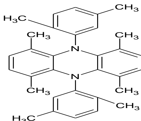
(III) 6,13-bis(2,5-dimethylphenyl)-dibenzo[C,H]diazecine
