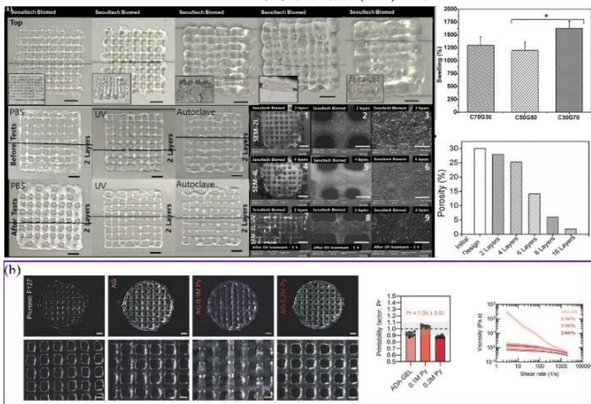
Fig. 5. (a) The C50G50 hydrogels are made of carboxymethyl cellulose (CMC) and glycol chitosan (GC). Images of 3D-printed samples with lattice structures before and after stability tests with PBS, UV irradiation, and autoclaving, digital pictures of the two-layer structures were taken. SEM pictures of samples with two-layer structures after UV treatment for one hour were also taken. The graphs on the right show the printed layers' strut diameters with the printed structures' length (mm) and porosity [46], and (b) Precursors of the conductive hydrogel ADA-GEL-Py
